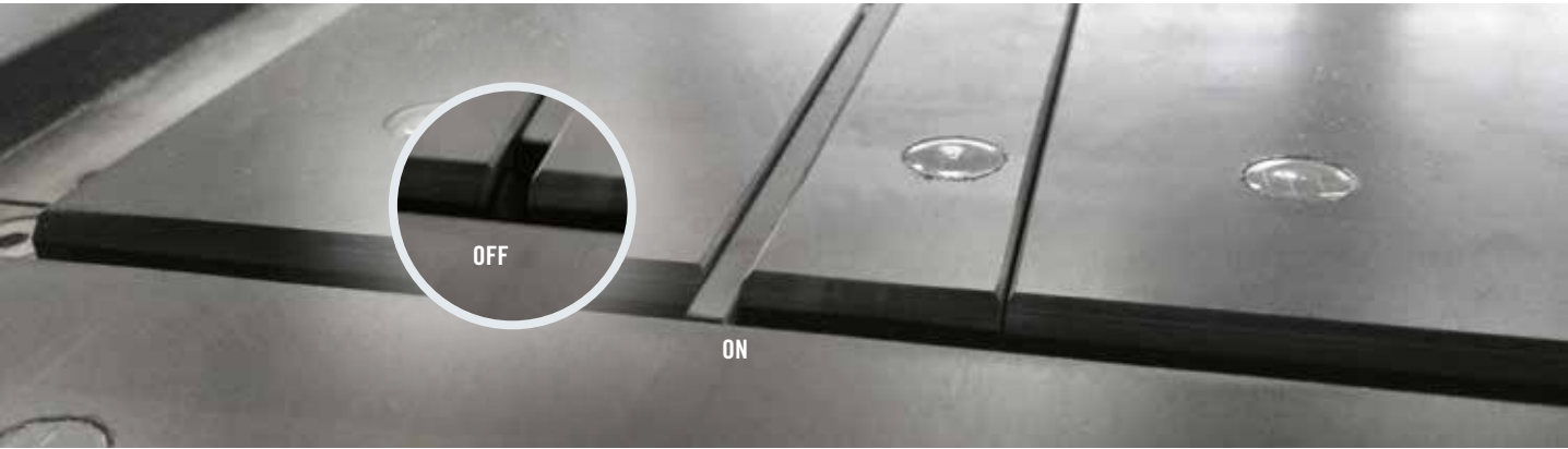
AUTOMATIC CLOSURE OF THE CUTTING LINE: it avoids the fall of waste trim cuts inside the machine.
