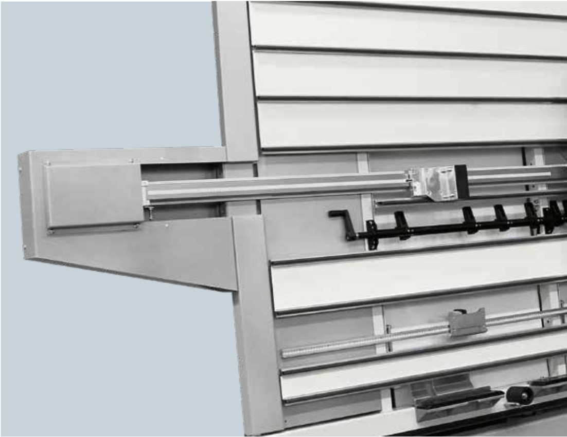
Posi-system: electronic stop for vertical cuts
